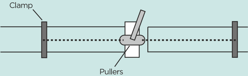
Figure 10 Installation of GRP pipe with puller
