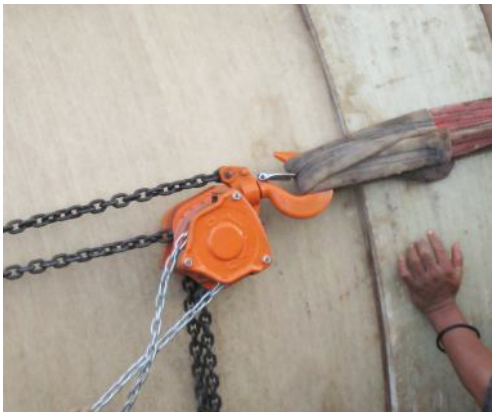
Figure 10 Installation of GRP pipe with puller
