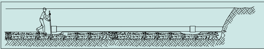
Figure 9 Installation of GRP pipe with lever
